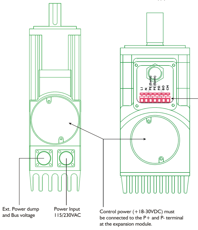
MAC400 supply connections
