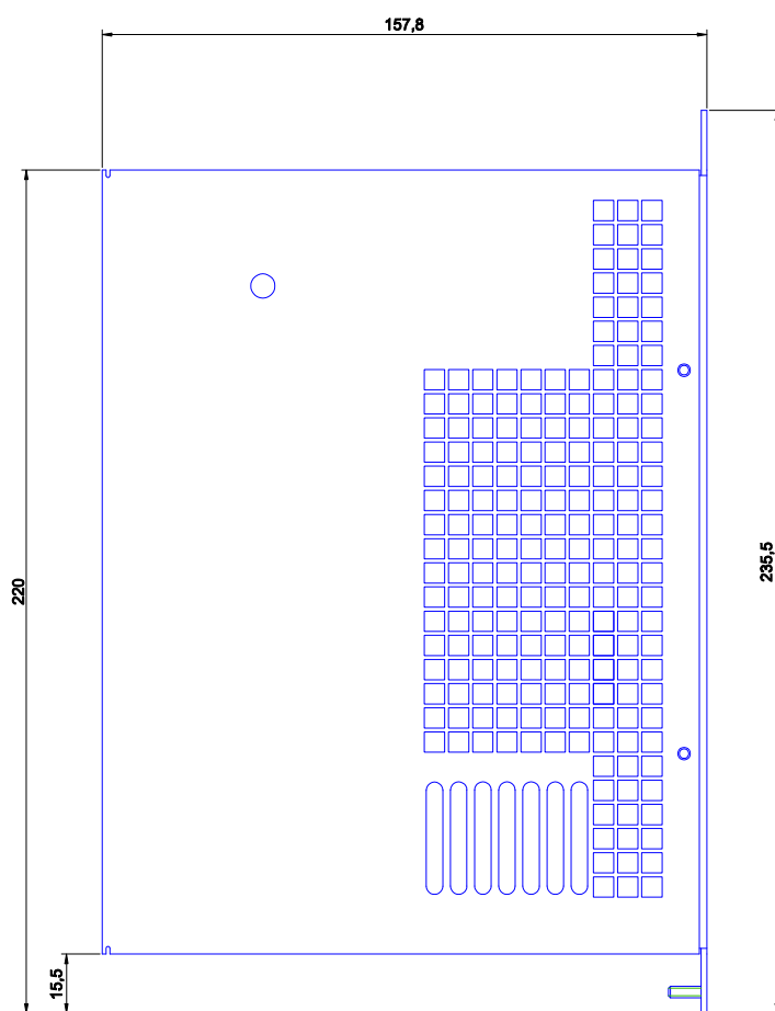
SIDE VIEW
