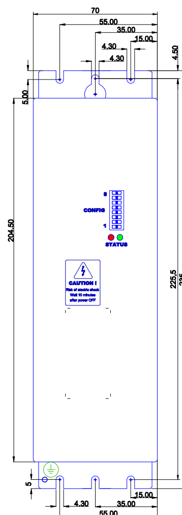
FRONT VIEW
