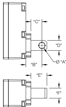
Rear Eye (KSRE-75, KSME-75)
